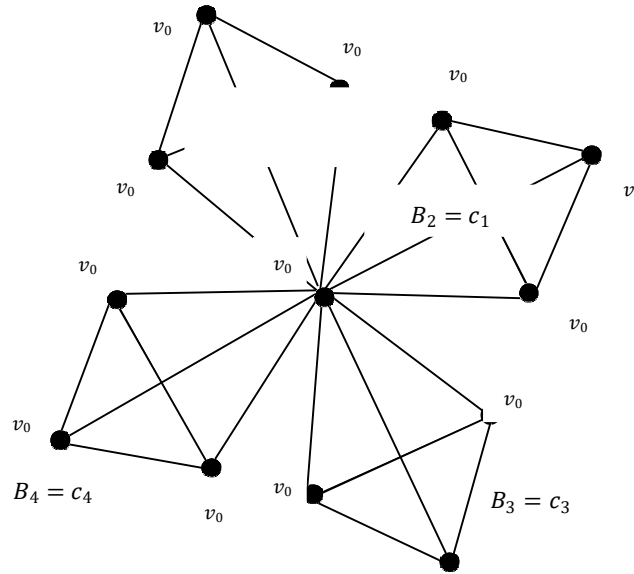
Fig 4: Windmill Wd(4,4)
